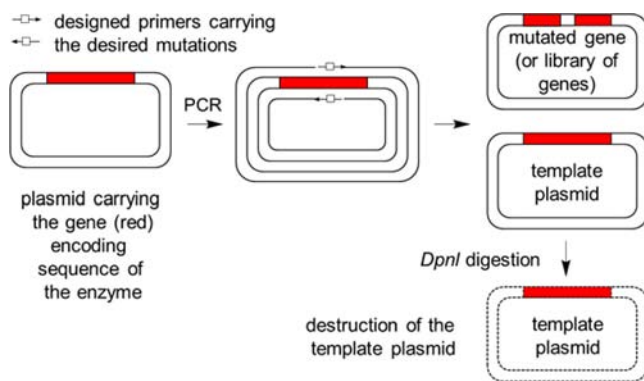
Figure 3. Steps involved in saturation mutagenesis according to the QuikChange protocol, adapted from ref 28.
